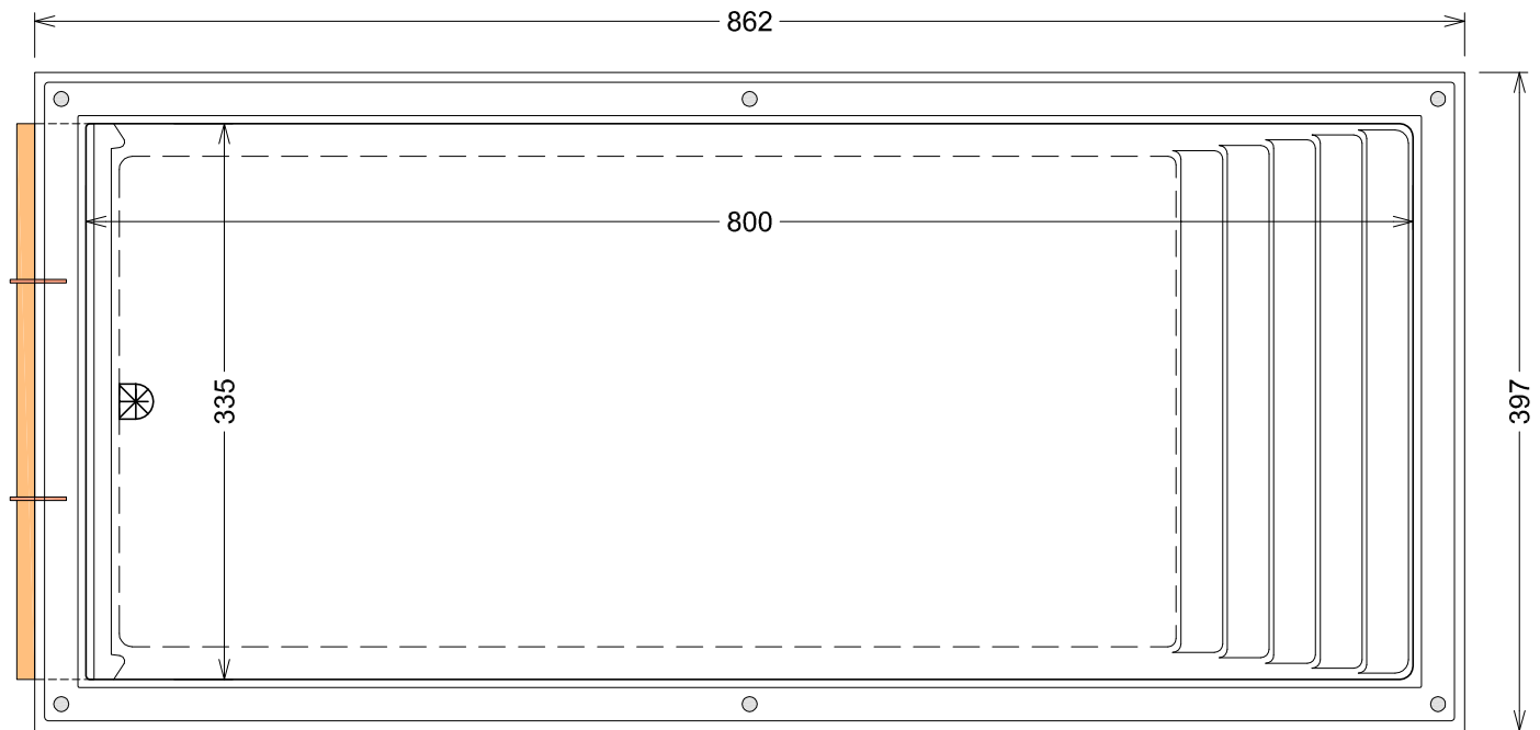
Grundriss - Ground plan
