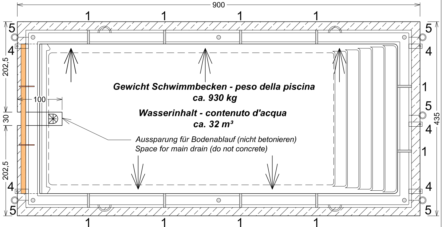
Grundriss - Ground plan
